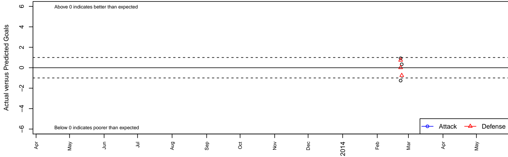
Scottsdale 01 Blackhawks B00 Dots are actual minus expected GF (blue circles) and GA (red triangles). Blue line is smoothed change in attack strength. Red is smoothed change in defense strength.
